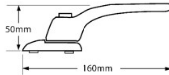
CHAMELEON Adaptable Inline Window Espag Handle (15mm – 55mm)
