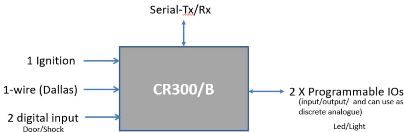
Figure 1 – IOs
