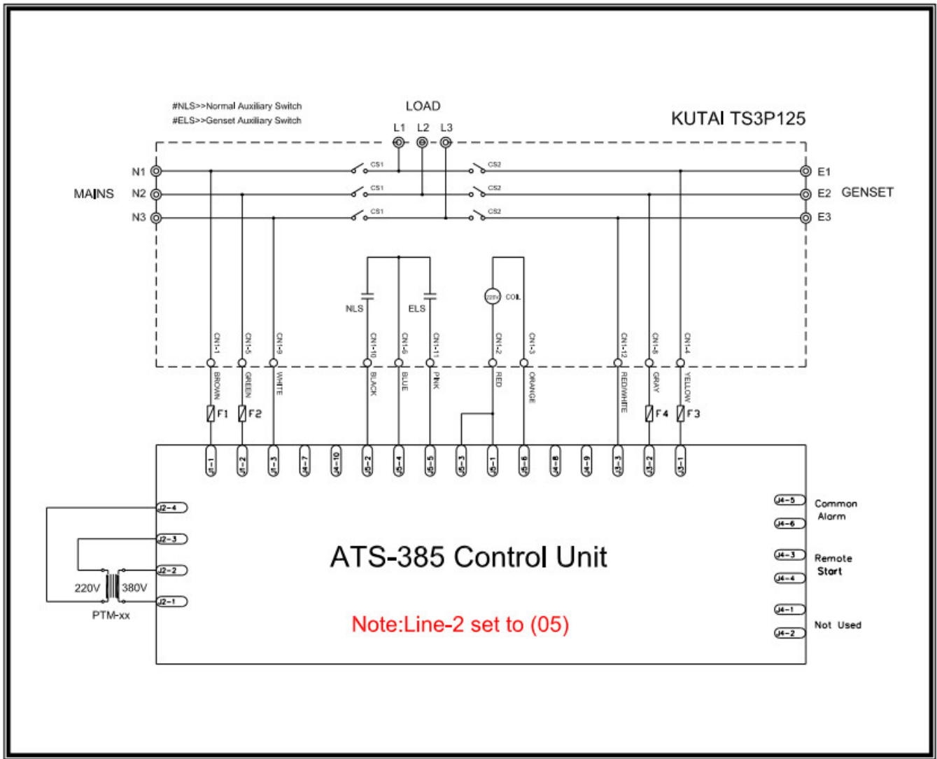
Magnetic Contactor Type ATS Wiring Diagram (3P/4P)
