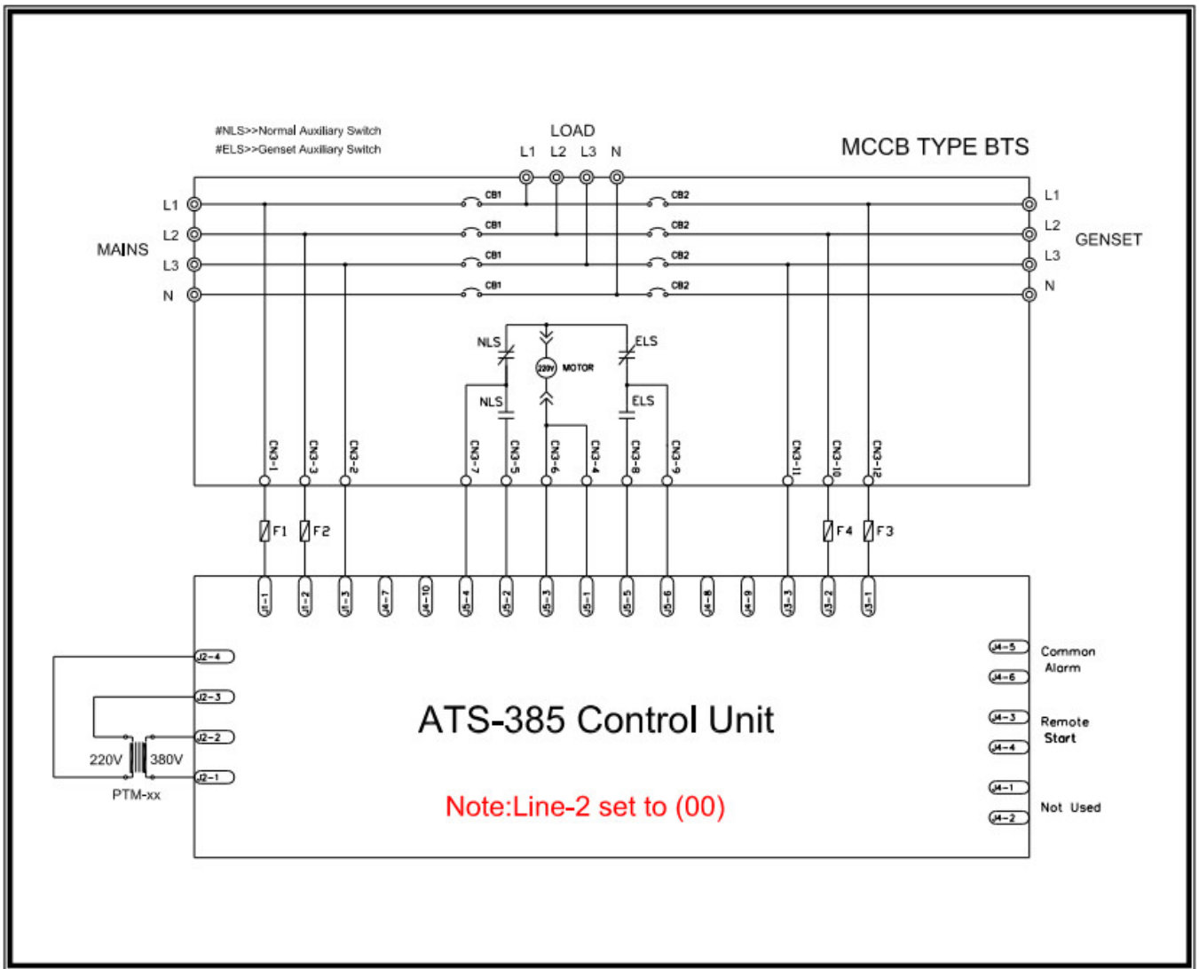
MITSUBISHI MD Type ATS Wiring Diagram (3P/4P) — MCCB With Separate Motor
