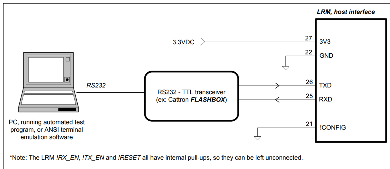
Figure 5.1 – LRM2 connection for stand-alone operation
