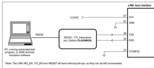
Figure 5.1 - LRM2 connection for stand-alone operation
