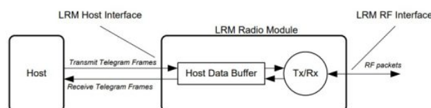
Figure 4.2 - Data communication model
