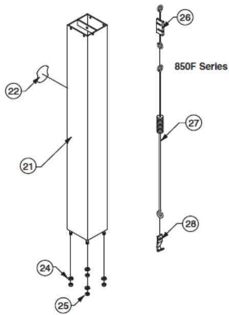
Figure No. 5 Column Assembly Parts Diagram
