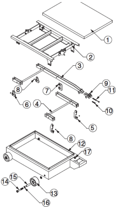
Figure No. 4 Scale Base and Parts Diagram Models 585XF and] 885XF
