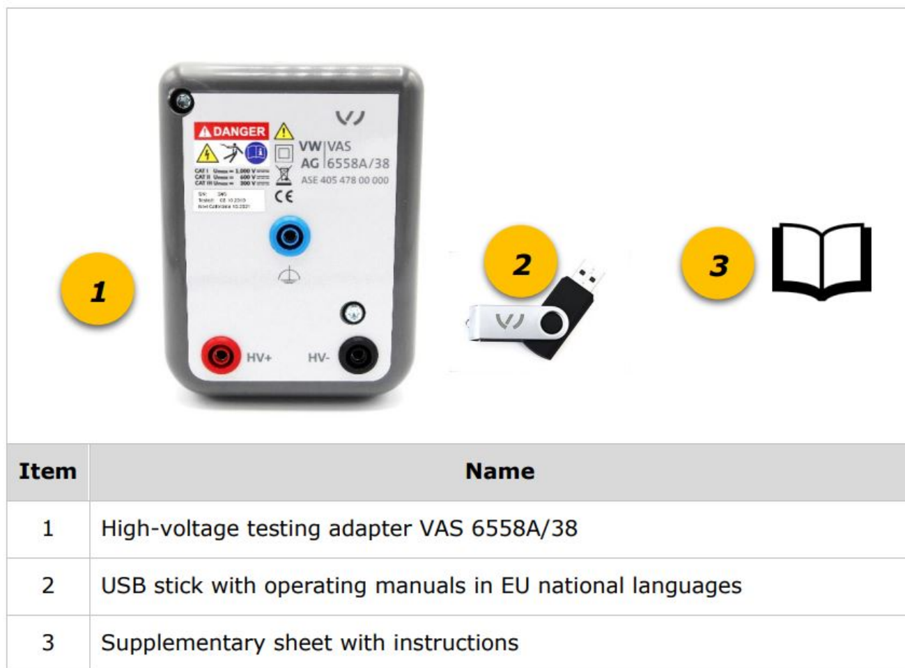
Fig. 1: Scope of supply of VAS 6558A/38
