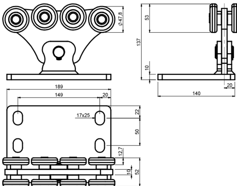
EIGHT WHEELED CARRIAGE FOR CANTILEVER GATE
