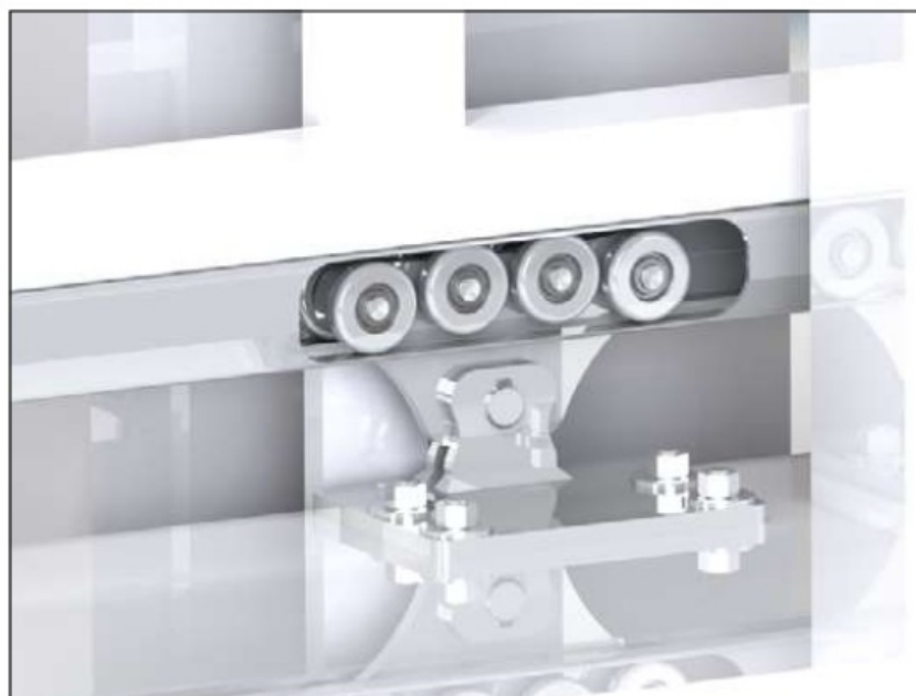
EIGHT WHEELED CARRIAGE FOR CANTILEVER GATE
