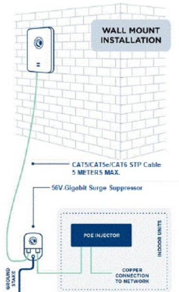
Figure 2 Grounding and lightning protection on wall
