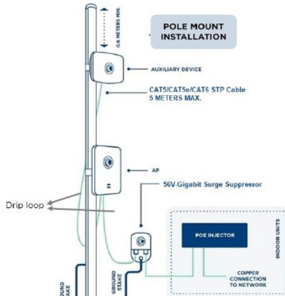
Figure 1 Grounding and lightning protection on pole or tower
