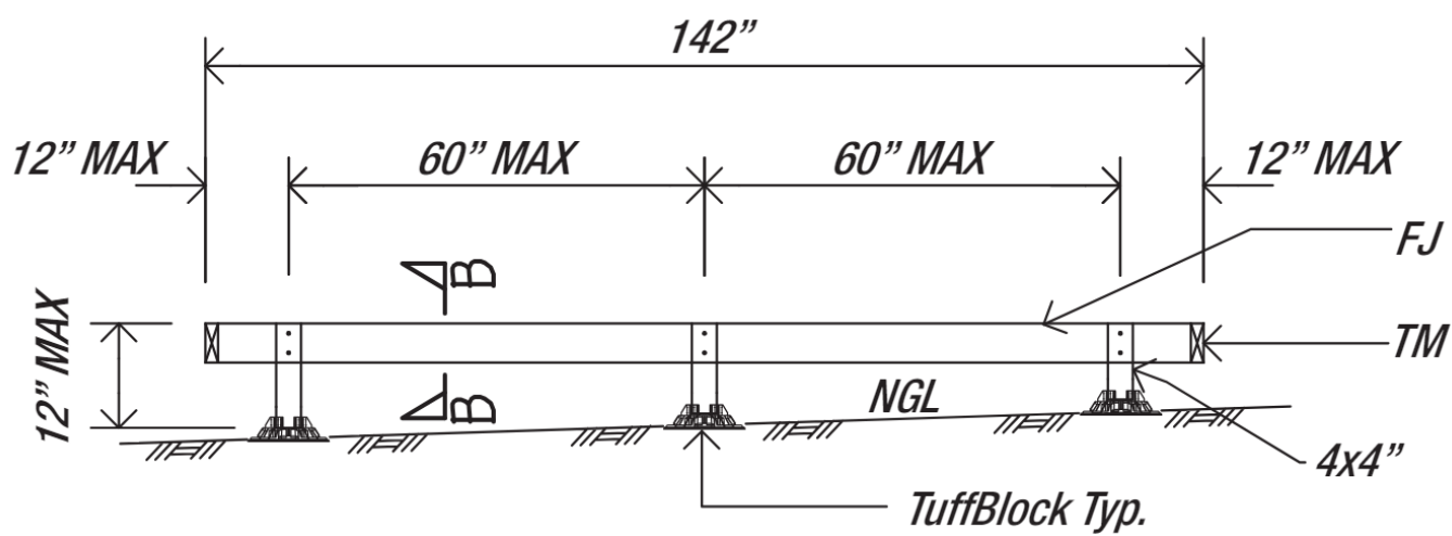
Section B-B
