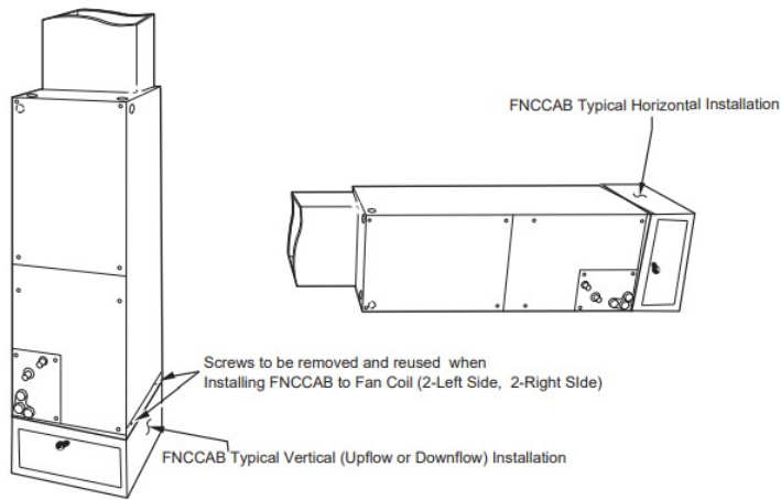
Fig. 4 – Typical Installation
