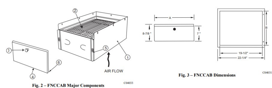
Fig. 2 – FNCCAB Major Components
