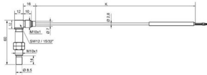
Figure 3-2) Dimensions IN-083
