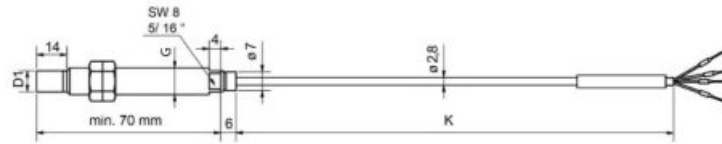
Figure 3-1) Dimensions IN-081
