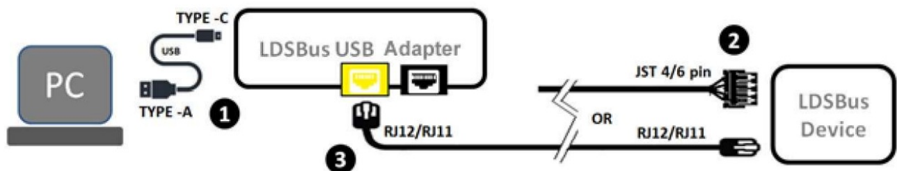
Figure 2 – LDSBus Device Configuration - Connection Diagram
