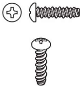
PHILLIPS PAN HEAD SCREW, 10-16 X 3/4 B100563 (4)
