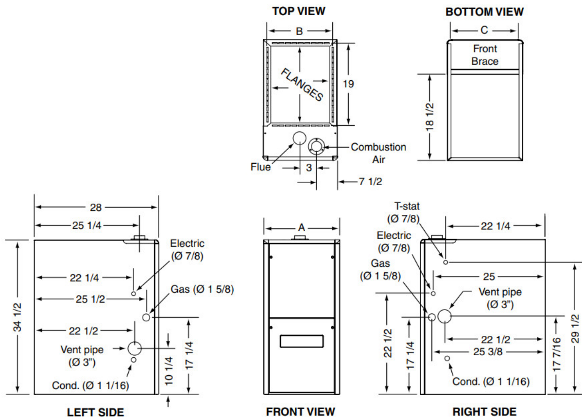
FG7TN 96% High Efficiency Downflow Series
