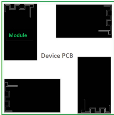
Fig 4 Optimal Position of Module
