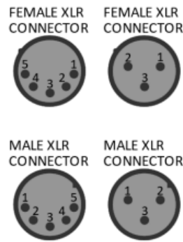
Figure 2: Remote Control connection pin-out and XLR connectors
