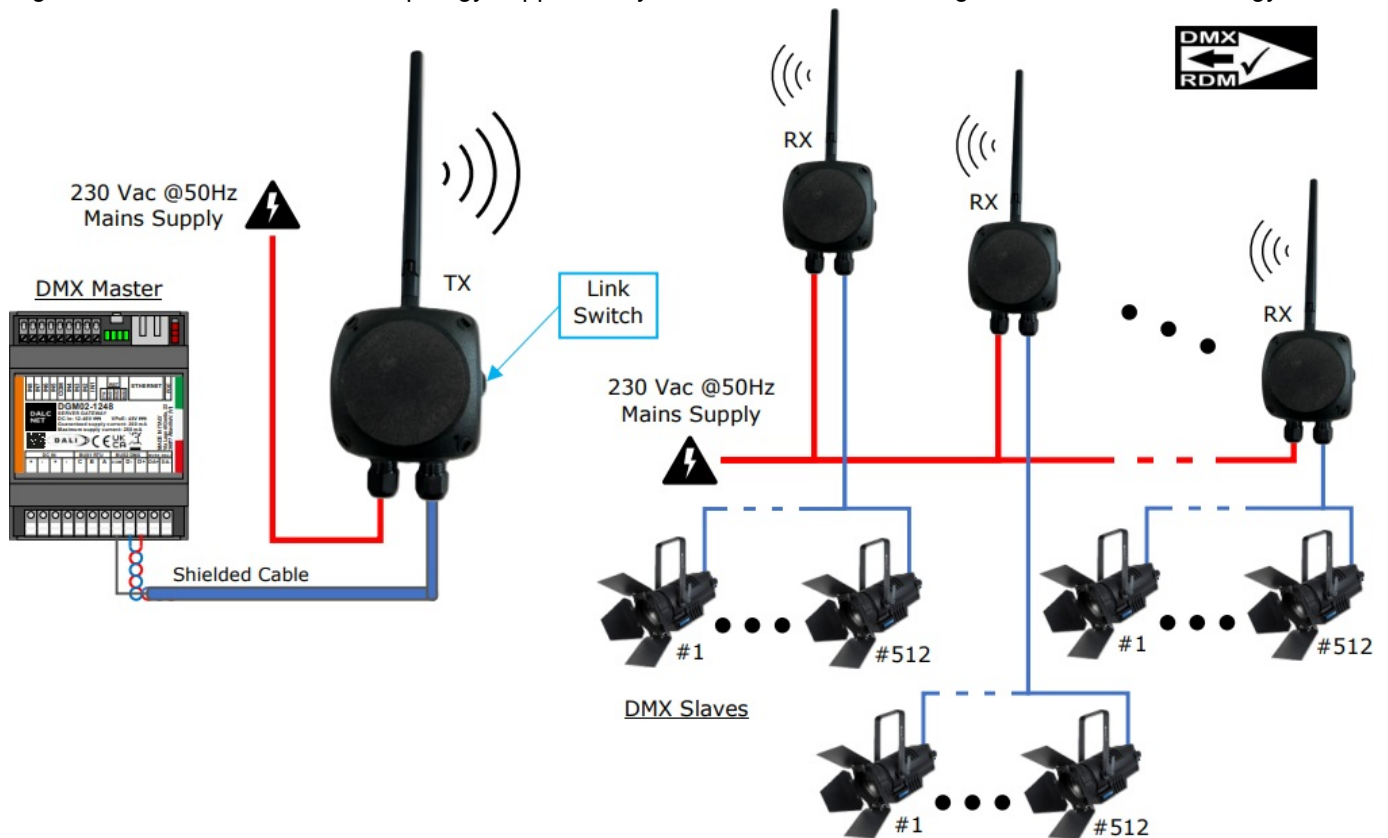
Figure 3: Remote Control Connection Topology
