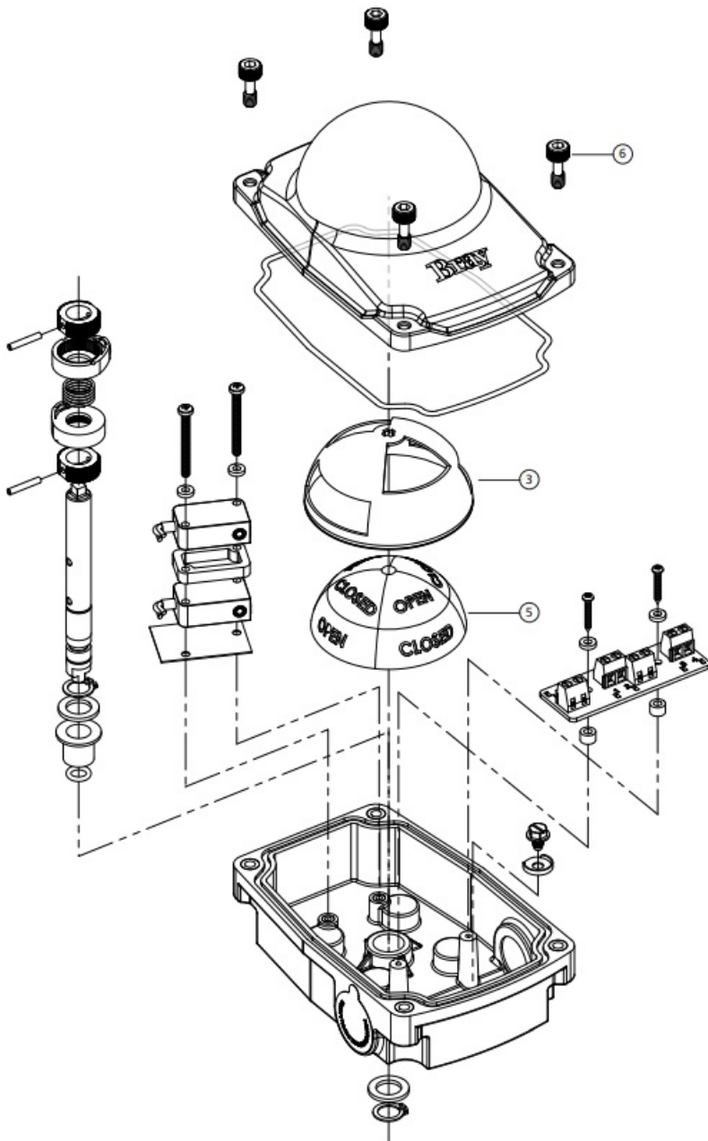
Exploded View – 5B Aluminum Trim
