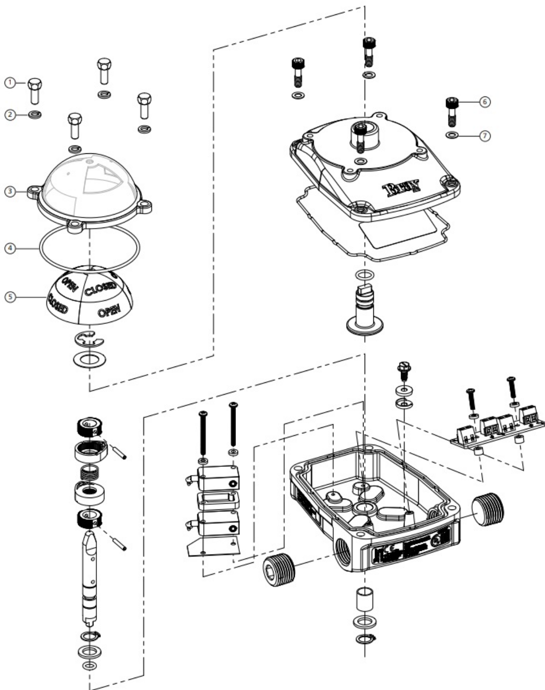
Exploded View – 5A – Resin Trim
