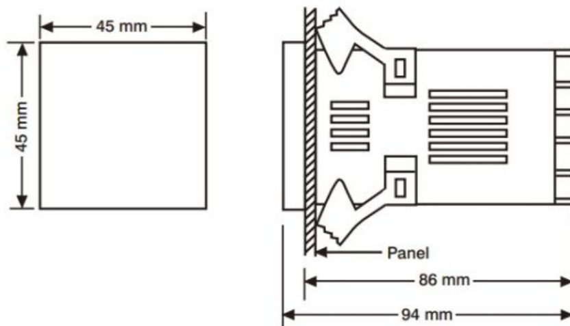
Figure 6.1 Mounting Dimensions
