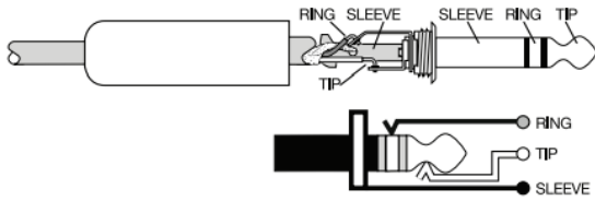
TRS balanced
