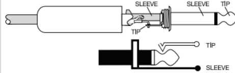
TS unbalanced
