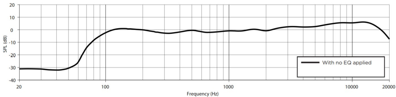
AMU206 Frequency Response
