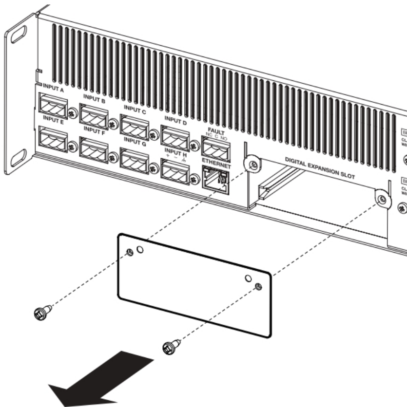
Fig. 1. Remove cover plate from rear expansion slot
