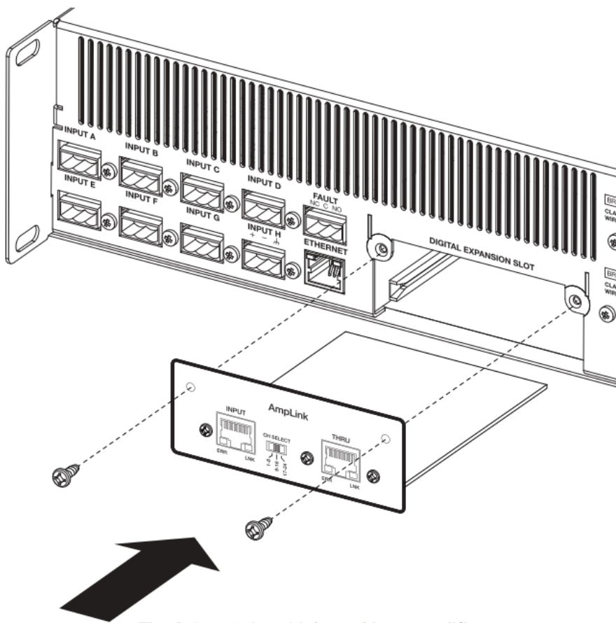
Fig. 2. Insert AmpLink card into amplifier
