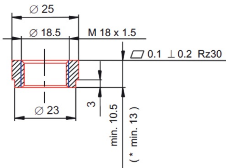
Fig. 7: Lambda Sensor thread boss Dimensions
