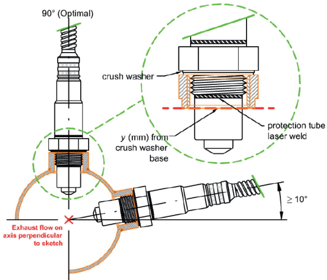
Fig. 6: Lambda Sensor Installation Diagram, Part 2
