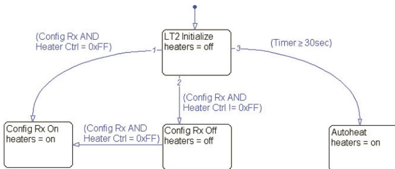
Fig. 4: CAN Messages Heater Control Strategy
