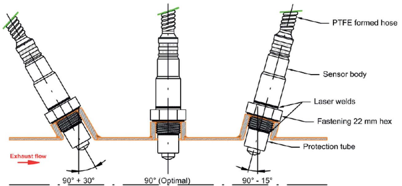
Fig. 5: Lambda Sensor Installation Diagram, Part 1
