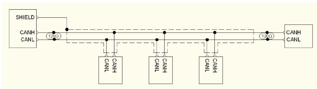
Fig. 3: Example of correctly configured CAN bus
