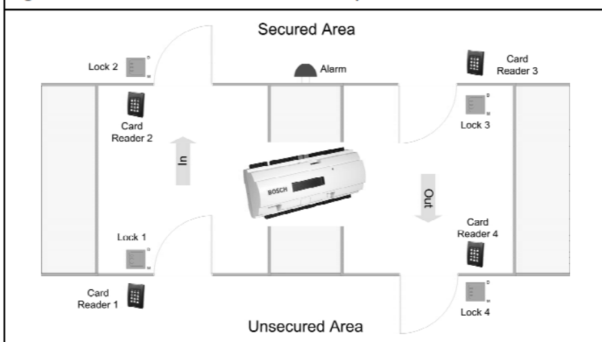
Figure 2: The AMC-4W in a four door safety lock
