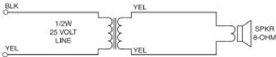
VRS1 Schematic Diagram
