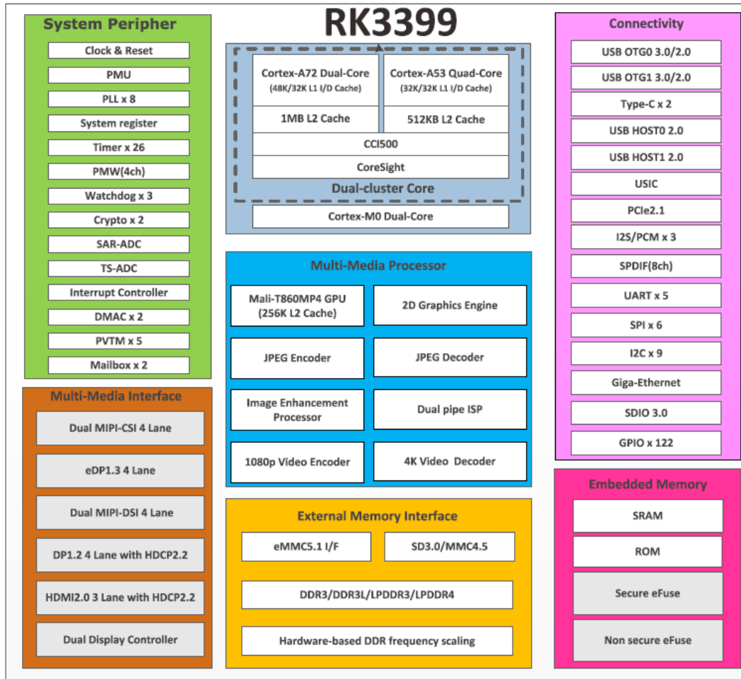
Block Diagram
