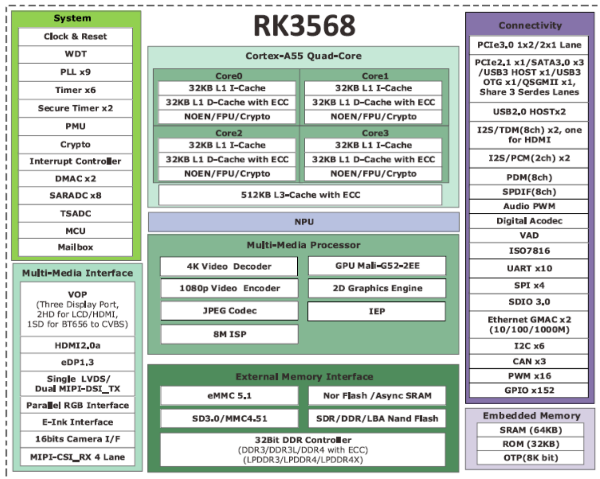
Development board Block Diagram
