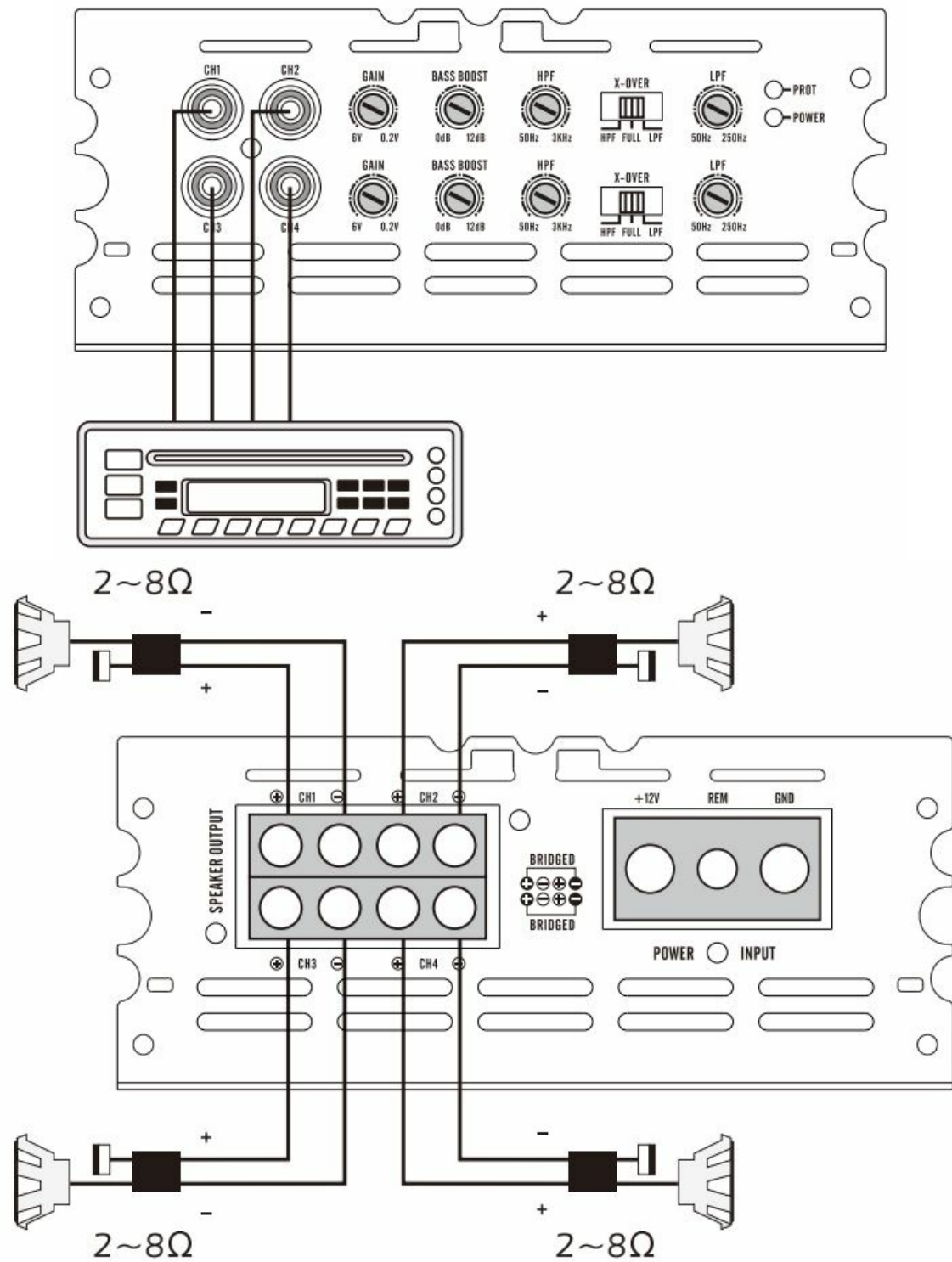
system 2: 3 channel mode
