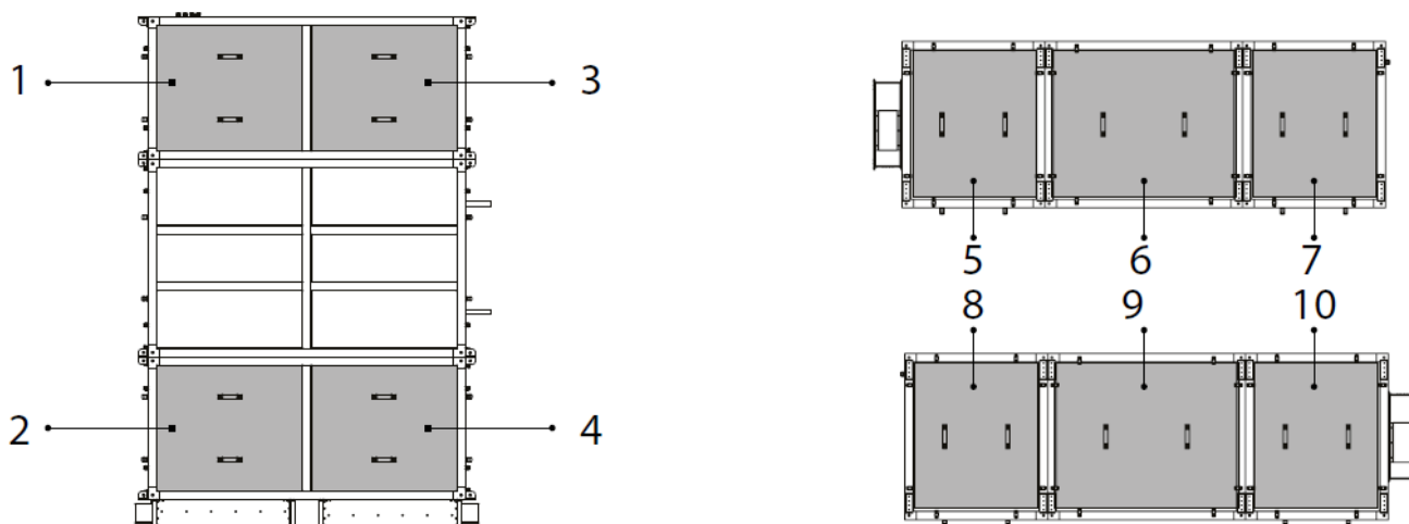
Service panels (CFP 5000/6000)
