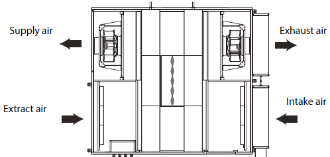
Left-sided modification (top view)
