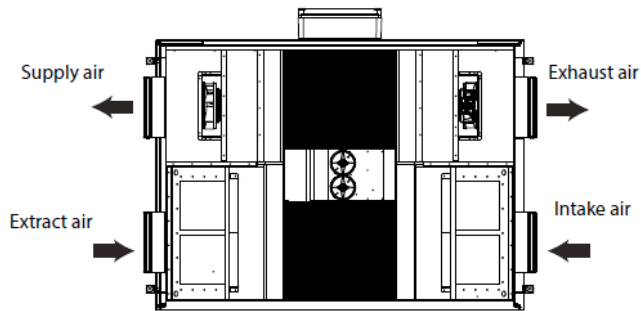
Left-sided modification (top view)
