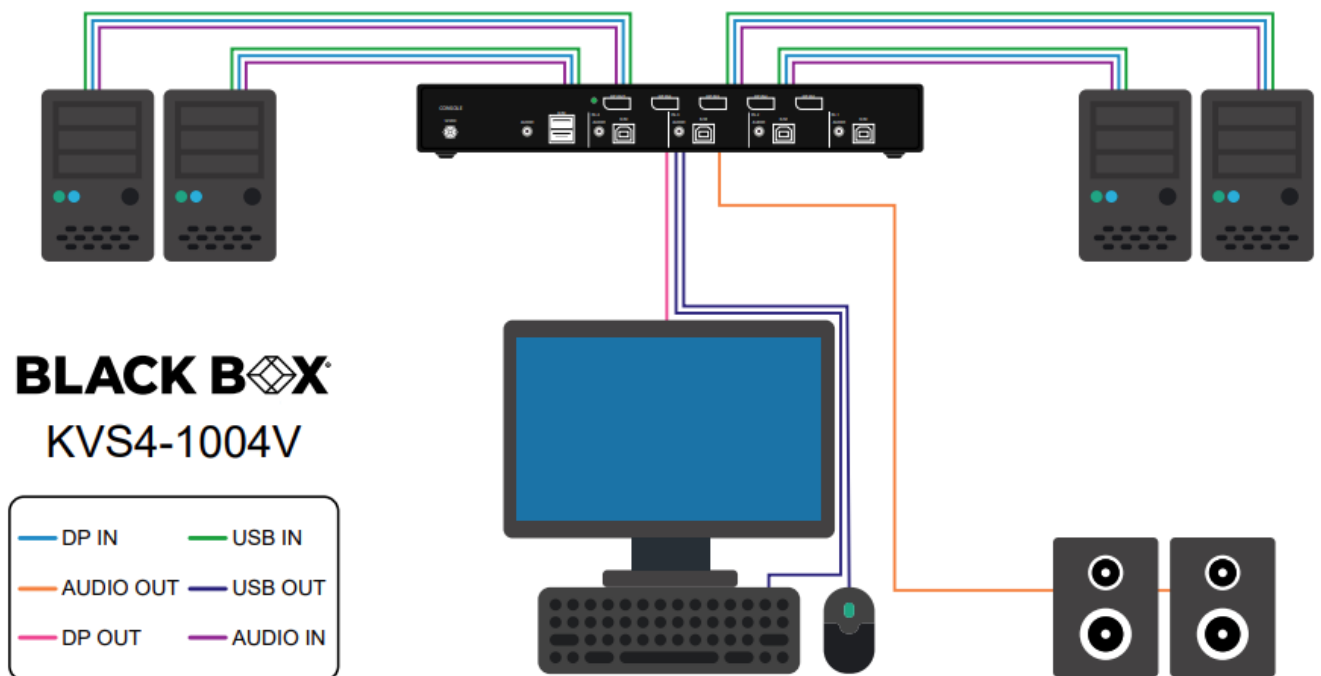
Figure 1-3: KVS4-1004V
