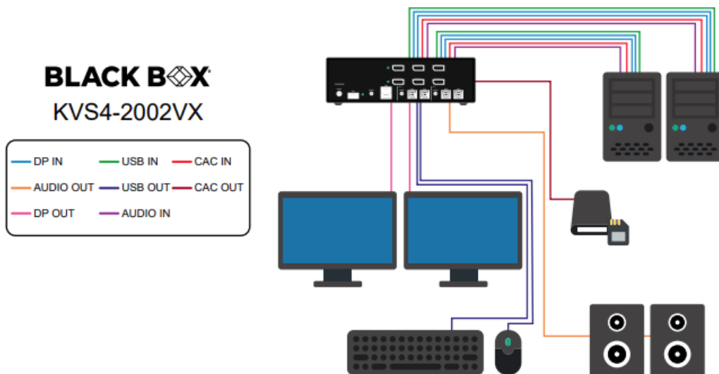
Figure 1-7: KVS4-2002VX
