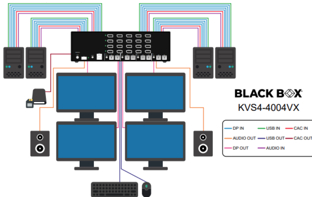
Figure 1-6: KVS4-4004VX
