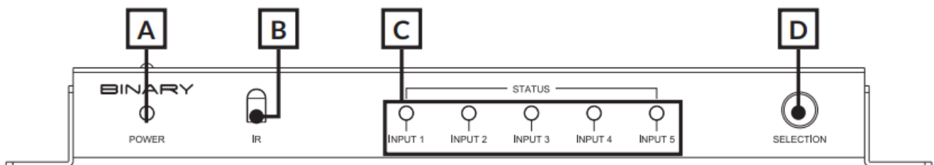
FIGURE 1: Front Layout
