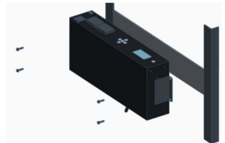
Surface Mount Step 2
