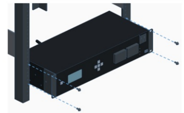
Step 3 Rack Mount
