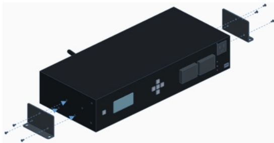
Surface Mount Step 1
