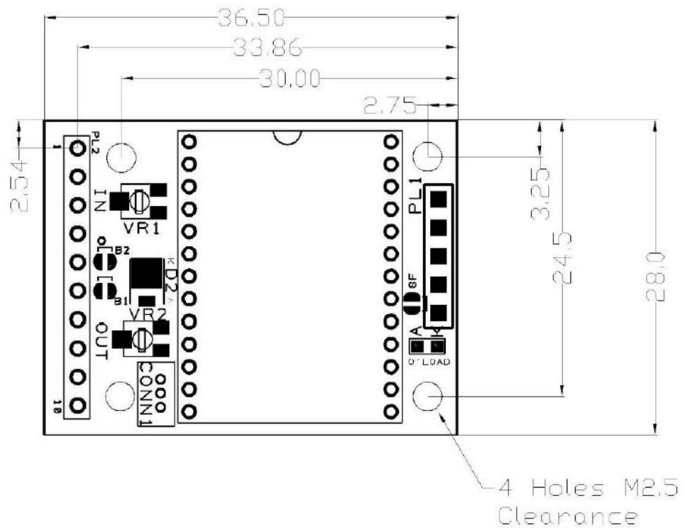
Figure 3. Board outline dimensions and mounting hole positions
