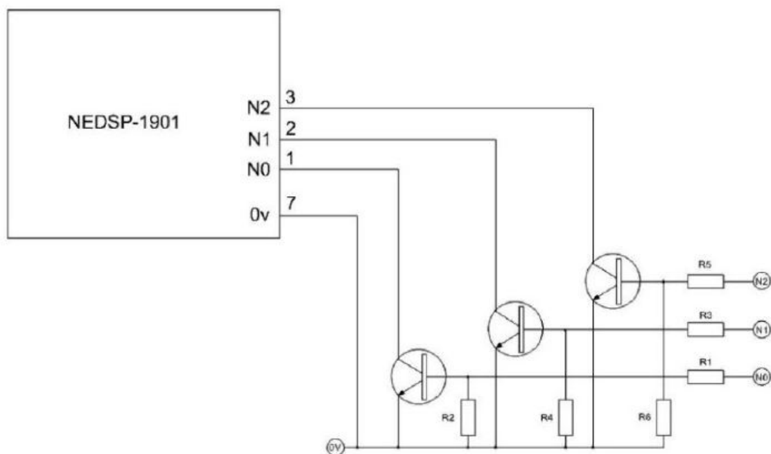
Figure 9. Noise Reduction setting using a Transistors
