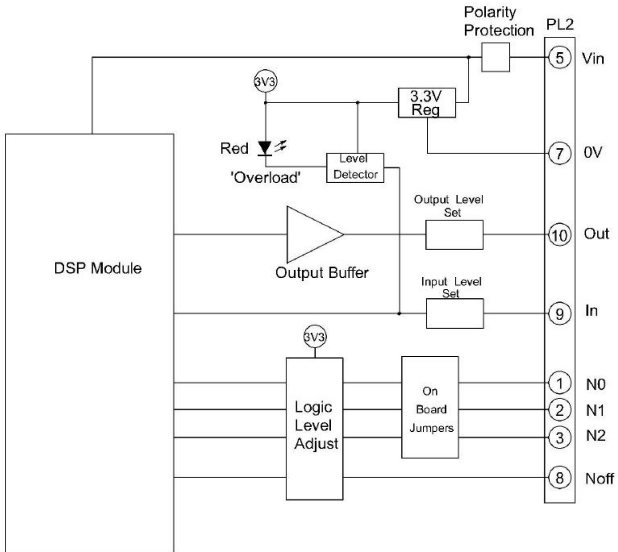
Figure 2. NEDSP1901 Block Diagram
