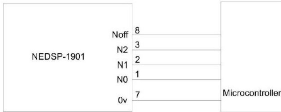
Figure 10 – Operation with a Microcontroller
