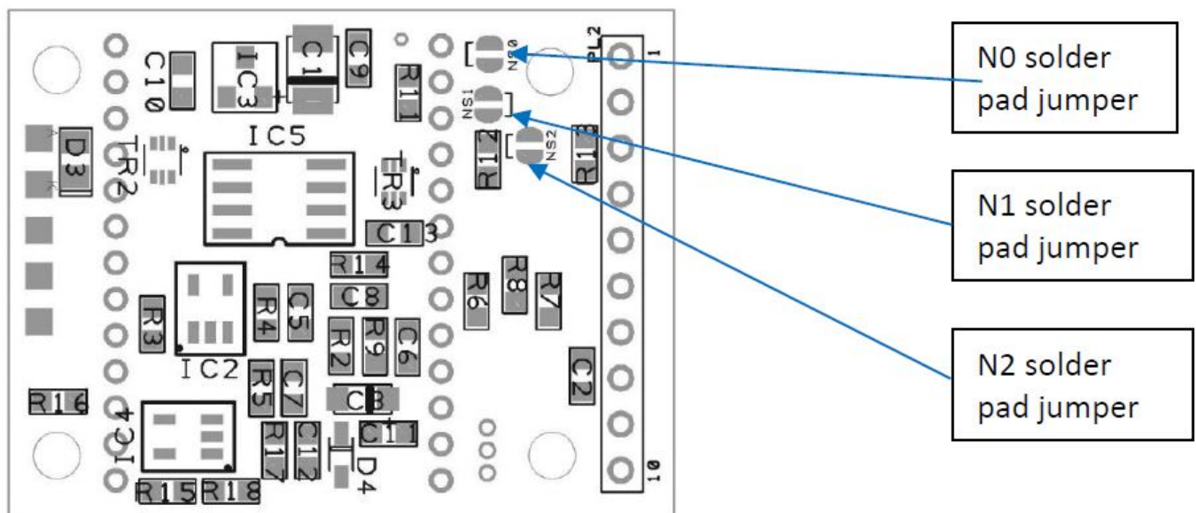
Figure 4. On-board Noise Reduction level selection jumpers
