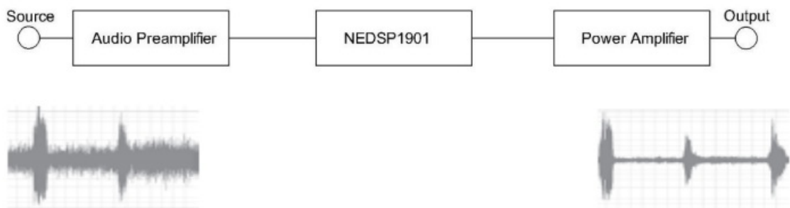
Figure5. General Audio signal flow with 1901 module installed
