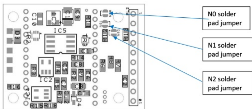
Figure 4. On-board Noise Reduction level selection jumpers
