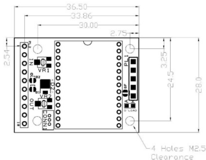
Figure 3. Board outline dimensions and mounting hole positions
