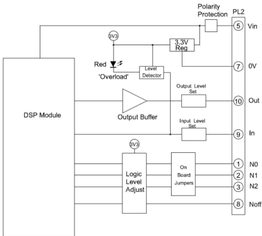
Figure 2. NEDSP1901 Block Diagram
