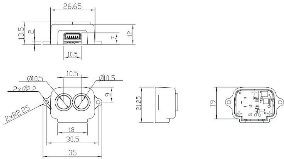
TF-Luna dimensions (Unit: mm)
