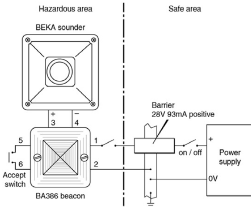
Fig 6 Combined beacon and sounder with alarm accept switch
