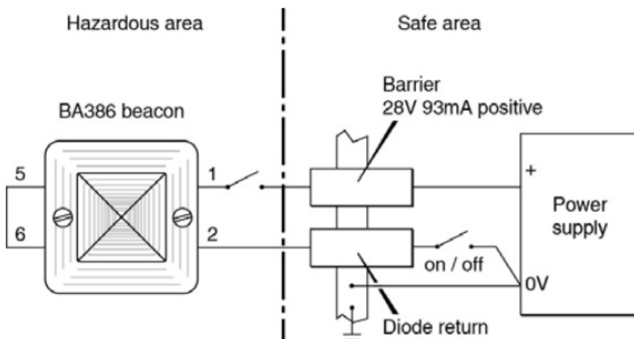
Fig 5 Single stage alarm using two channel barrier.
