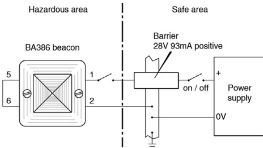
Fig 4 Using a single channel barrier.
