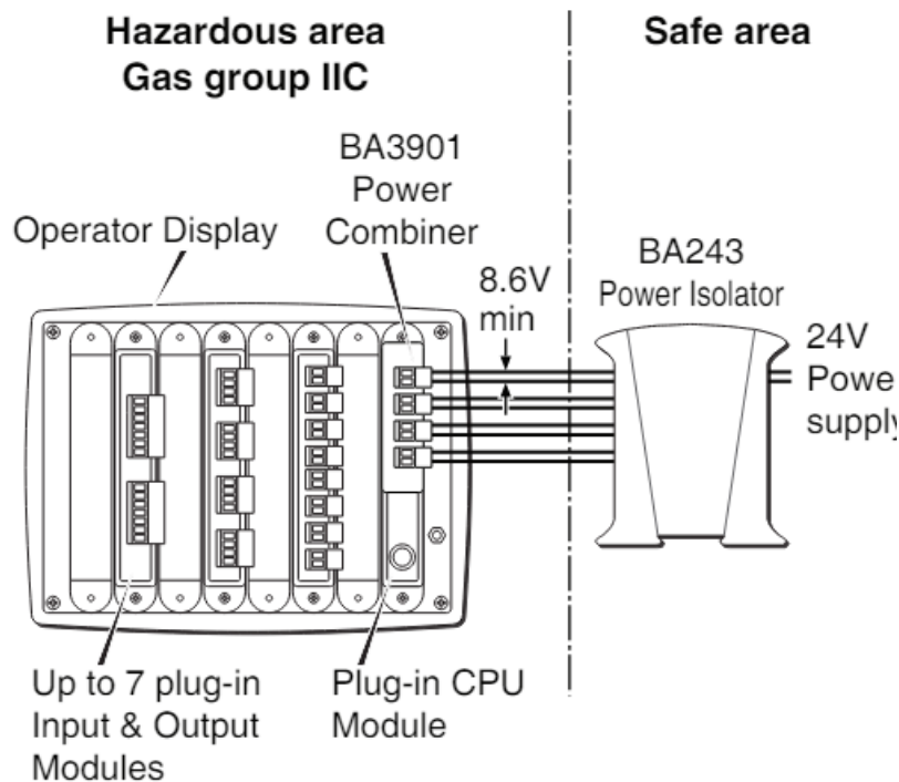
Fig 4 Application in gas group IIC
