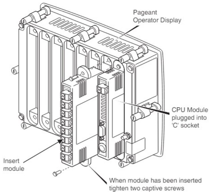
Fig 11 Installing plug-in modules
