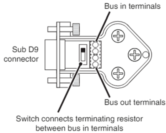
Fig 14 BA3903 RS485-IS SUB D 9 Connector
