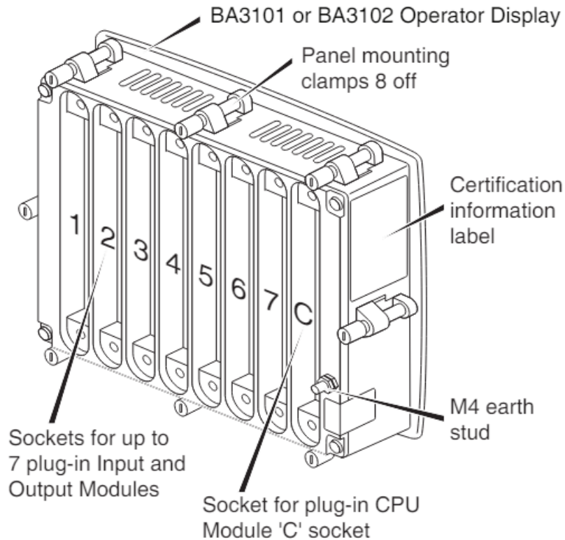
Fig 2 Rear of BA3101 display without plug-in modules
