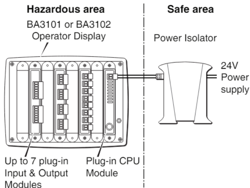
Fig 1 Pageant intrinsically safe Operator Panel system
