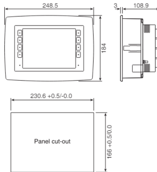
Fig 9 Pageant Operator Display dimensions including plug-in modules and panel cut-out.
