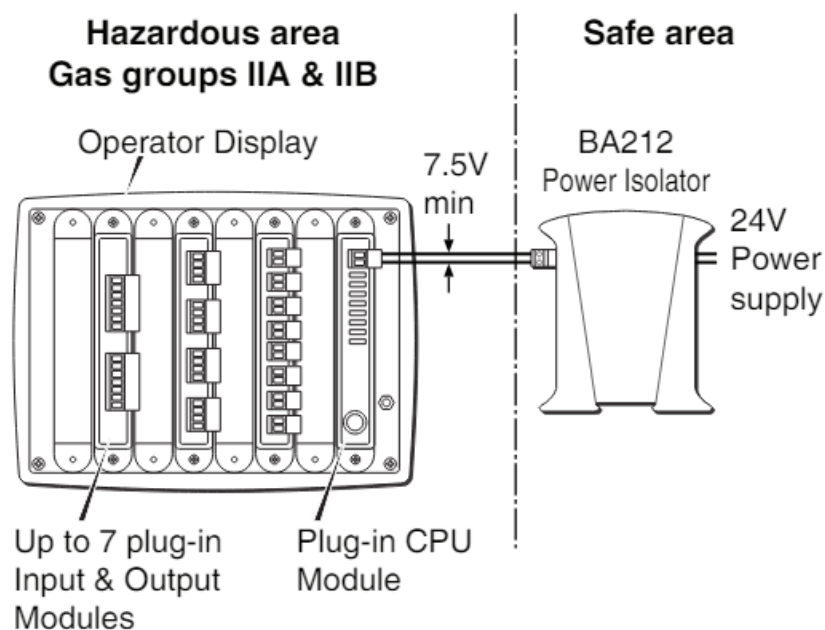
Fig 3 Application in gas group IIA or IIB
