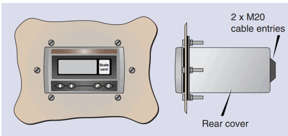
Fig 4 BA495 rear cover
