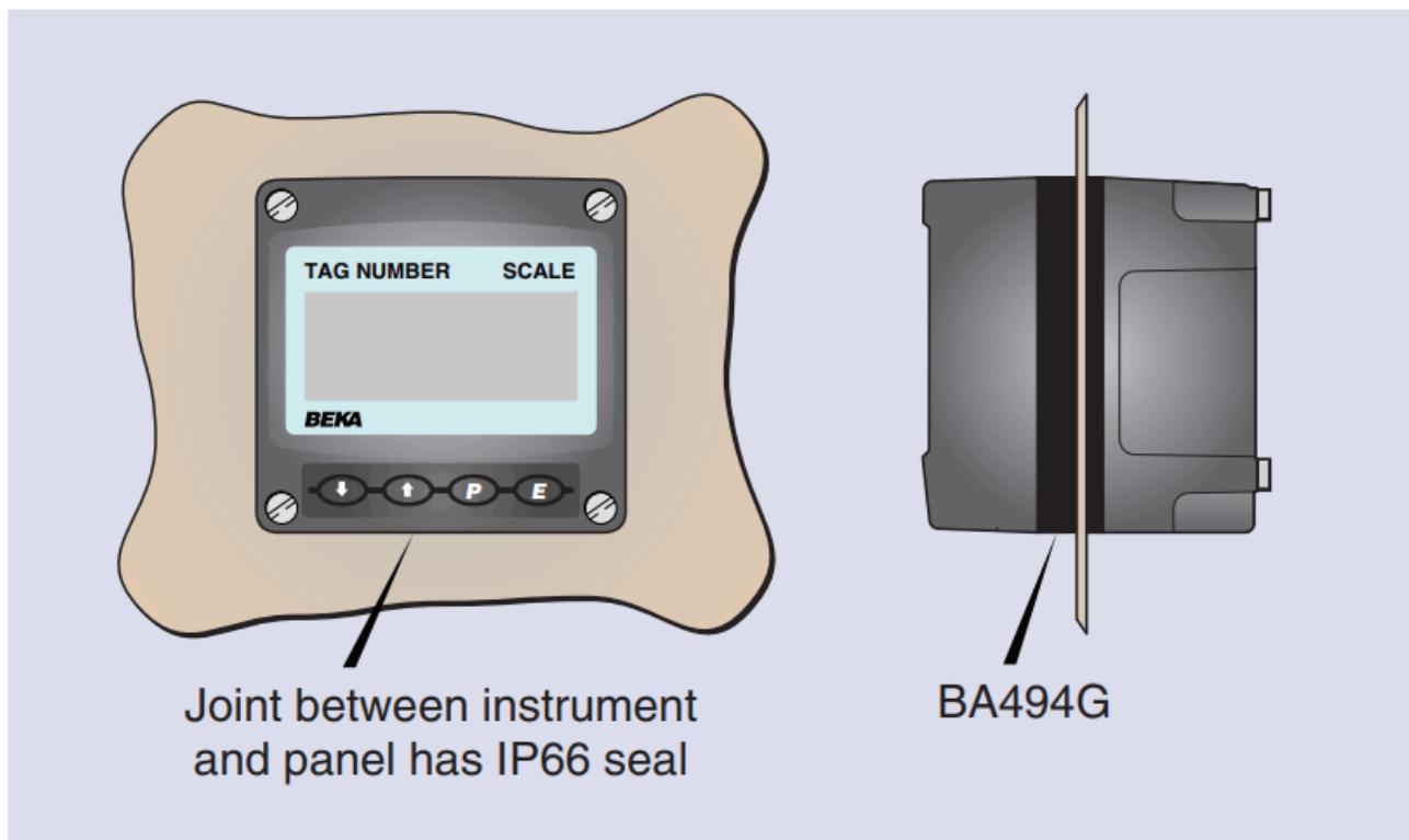
Fig 3 BA494G Sealed panel mounting kit
