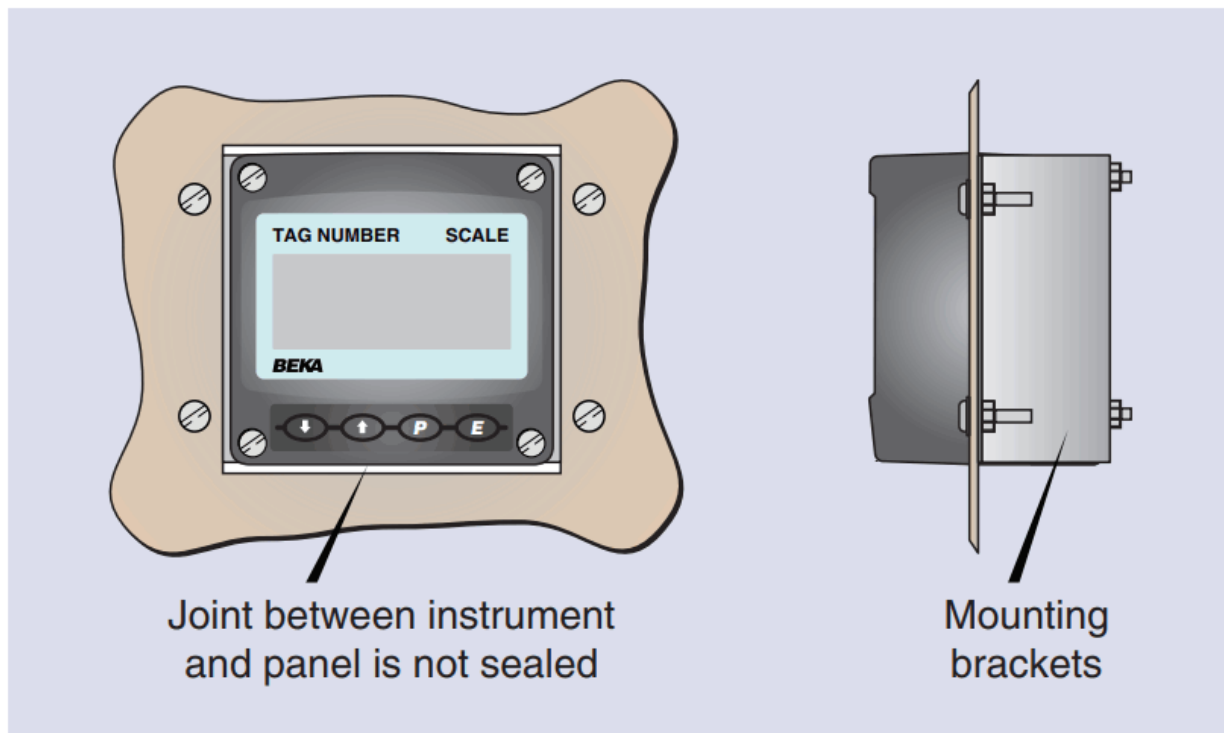
Fig 2 BA394G Panel mounting kit
