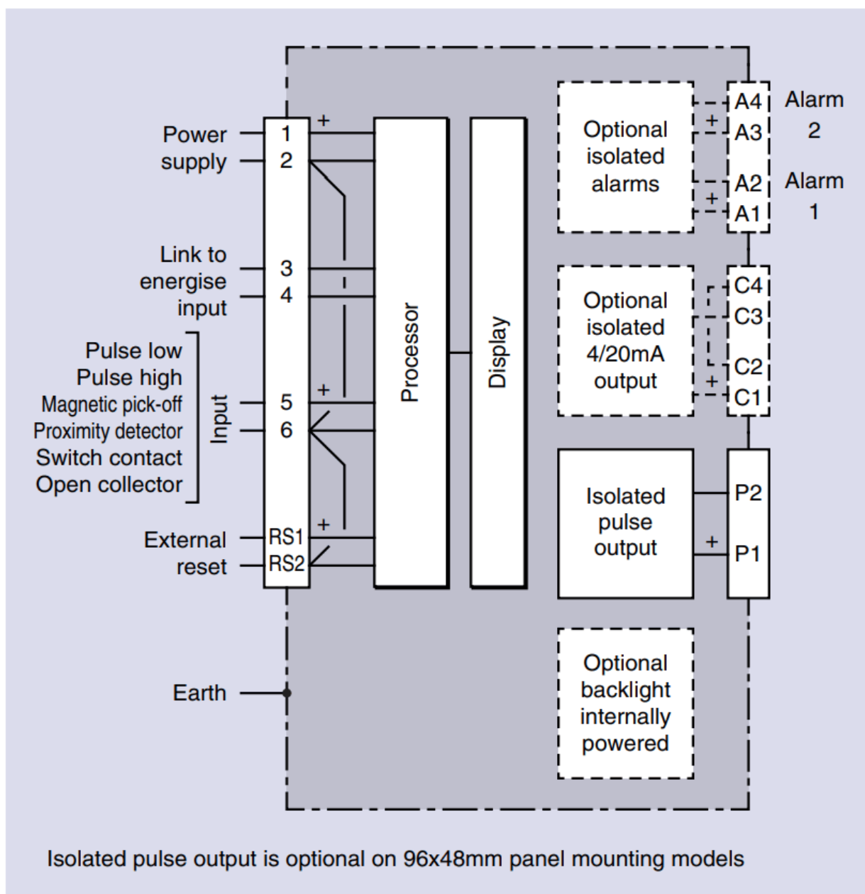
Fig 5 Simplified diagram of single input Rate Totaliser
