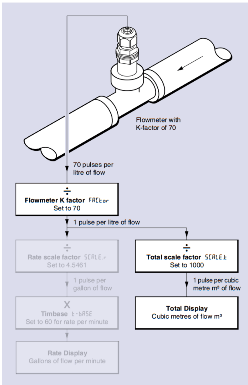
Fig 9 5scale . t set to 1000 to produce total flow display in cubic metres m³
