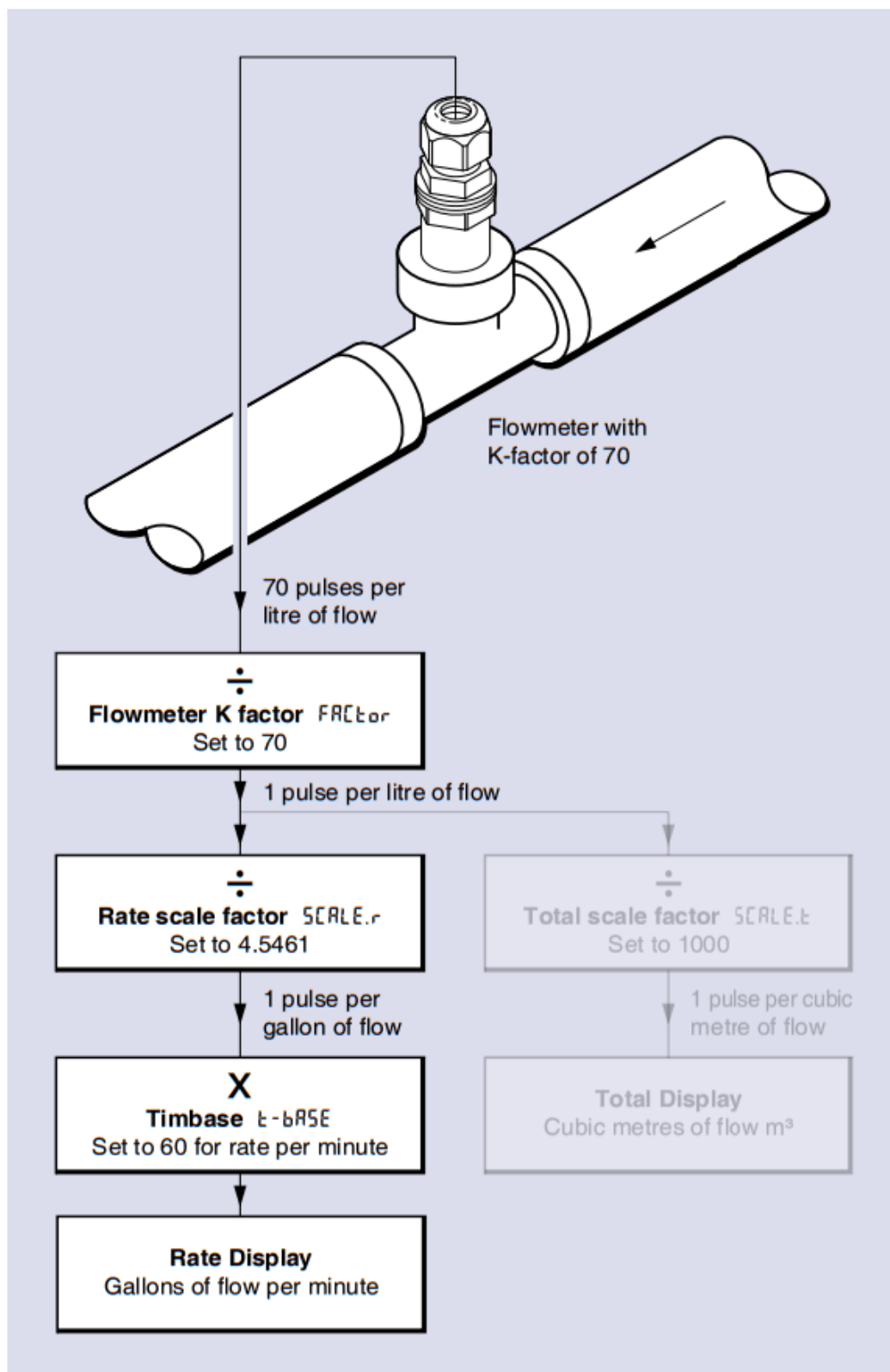
Fig 10 5scale r and t-ba5E set to provide a Rate Display in Gallons / minute
