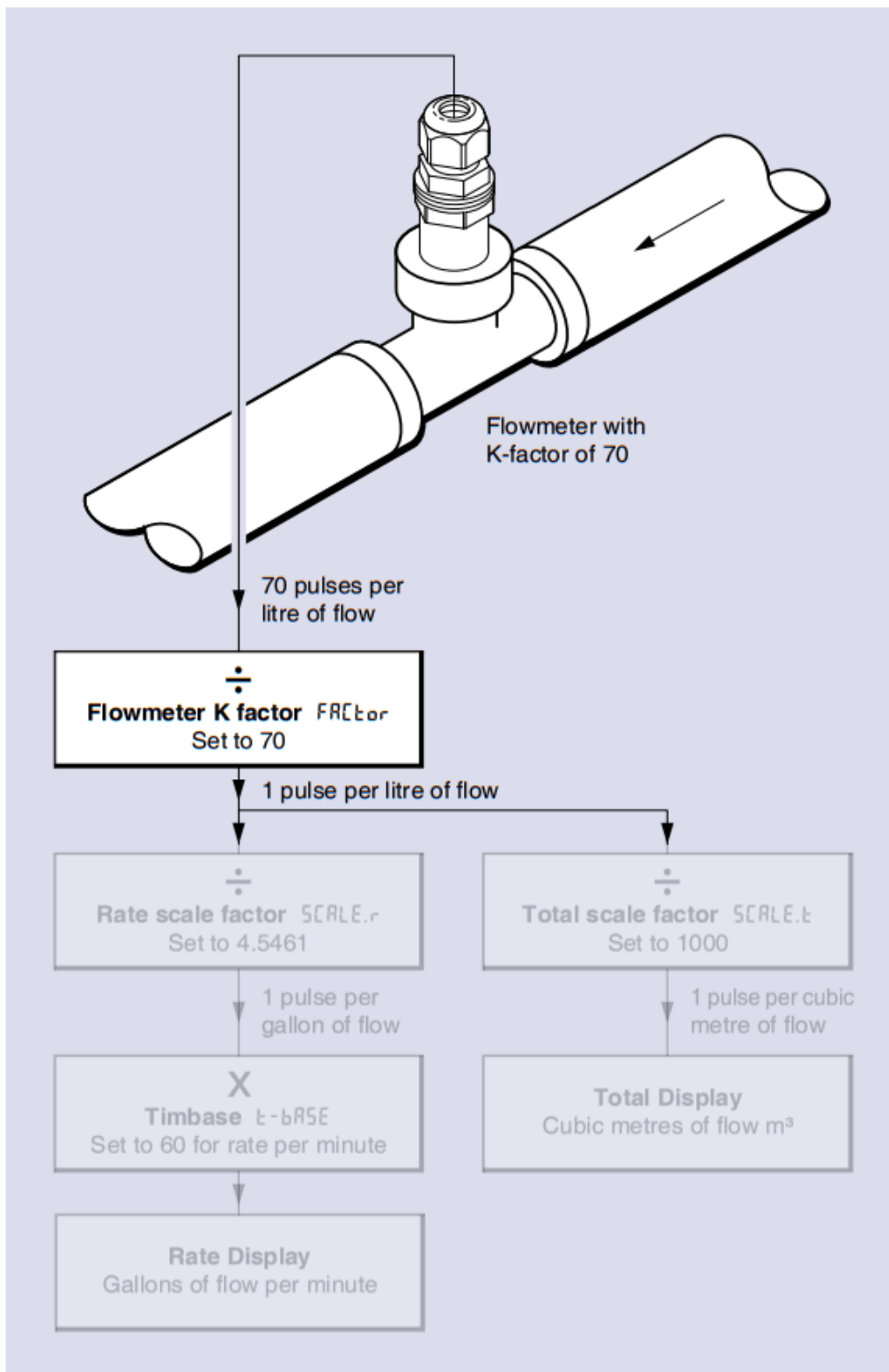
Fig 8 factor set to flowmeter K-factor
