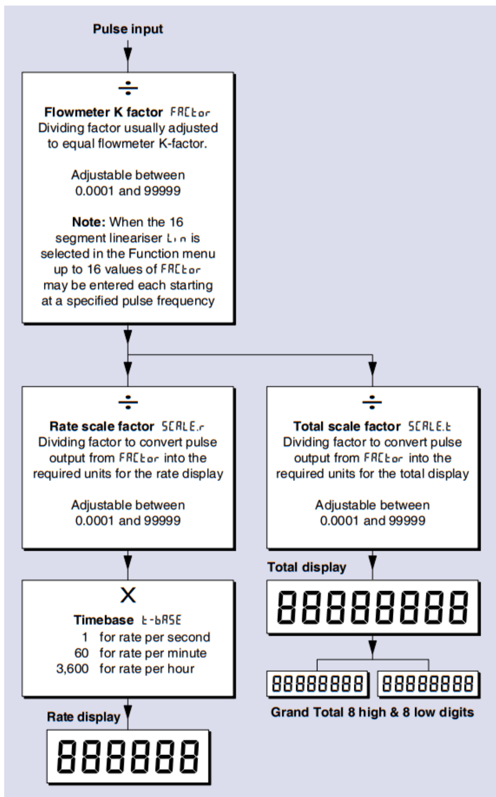
Fig 7 Single input Rate Totaliser Configuration structure
