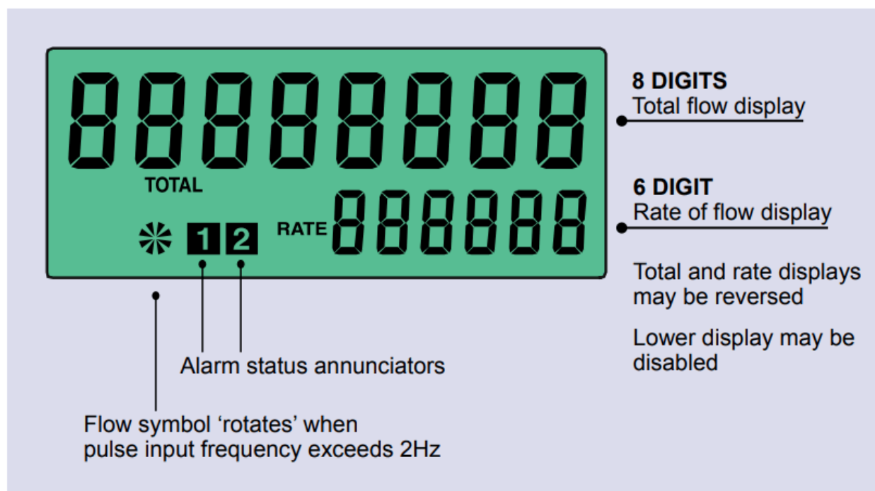
Fig 6 Rate Totaliser display
