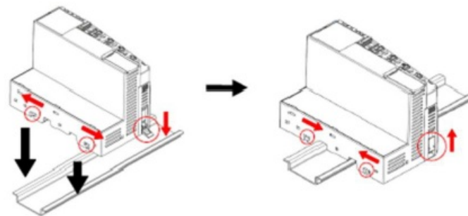
Mount to DIN rail
