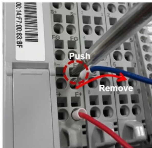
Disconnect cable
