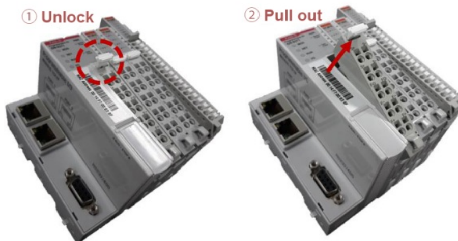
Dismount a removable terminal block
