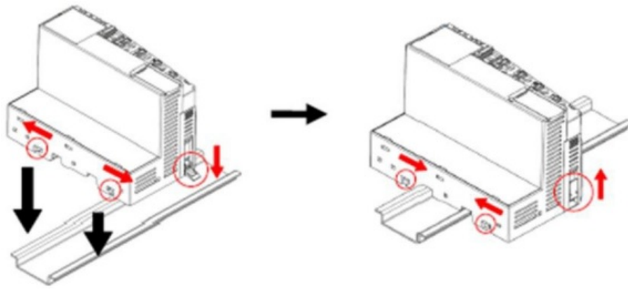
Mount to DIN rail
