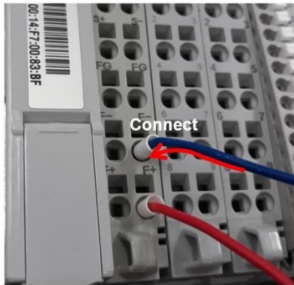
Connect cable
