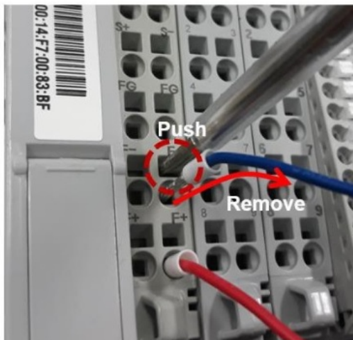
Disconnect cable
