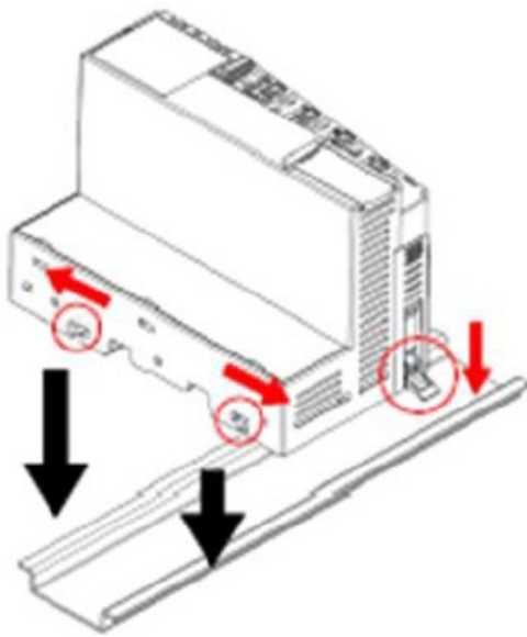
Mount to DIN rail
