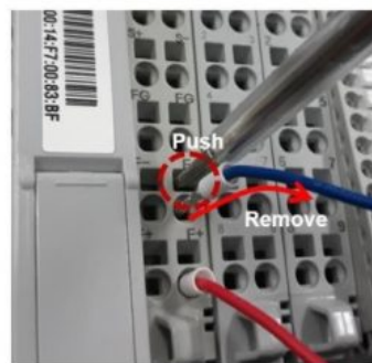
Disconnect cable
