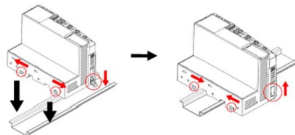
Mount to DIN rail
