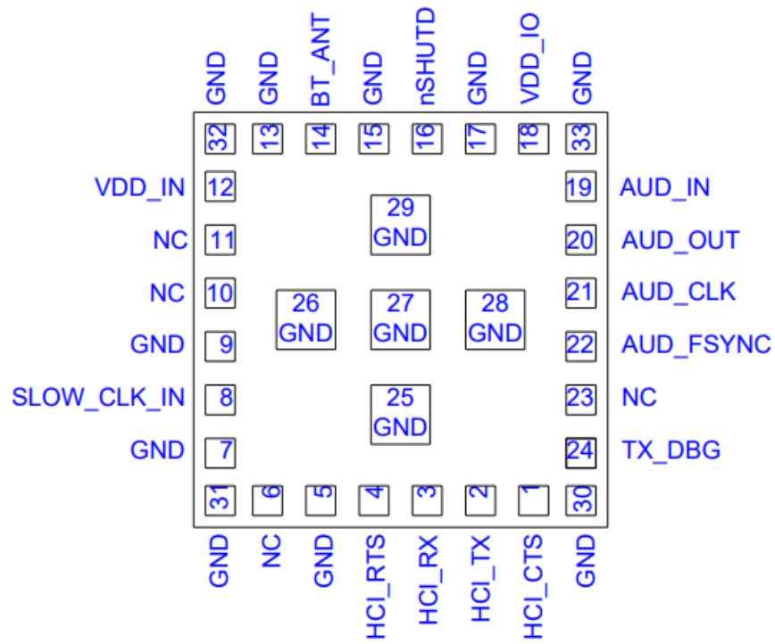
Bottom View
