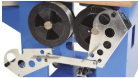
ESB 69-3 with two spool fixtures
