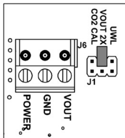
Fig. 7: J1 set for 0 to 5 VDC output
