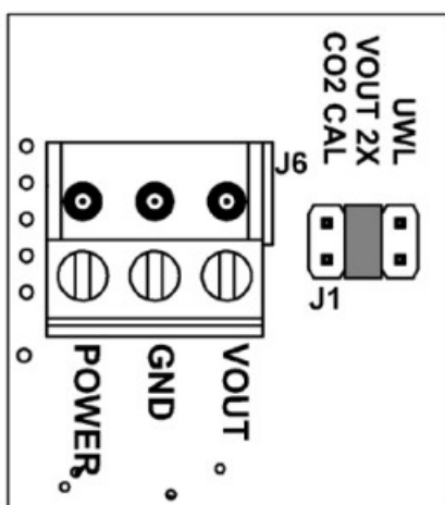
Fig. 6: J1 set for 0 to 10 VDC output
