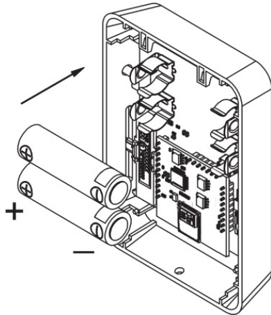
Fig. 6: Battery replacement
