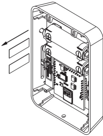
Fig. 2: Battery insulator tab removal
