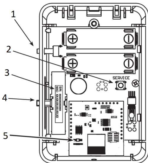
Fig. 5: Battery Powered BAPI-Stat “Quantum” Circuit Board with optional setpoint & override (The functionality is the same for wire power units.)
