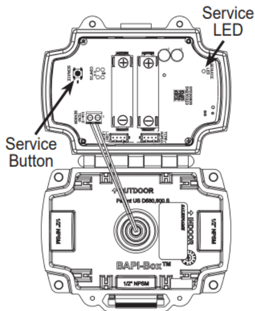
Fig. 8: BAPI-Box Sensor Service Button and LED
