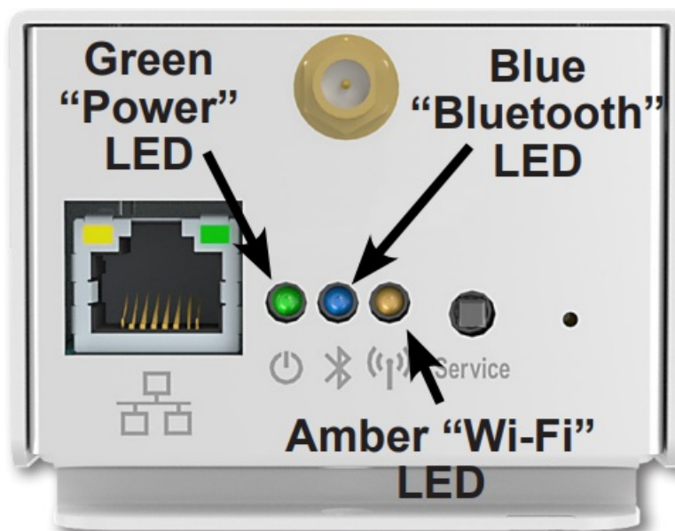
Fig. 11: Gateway LEDs
