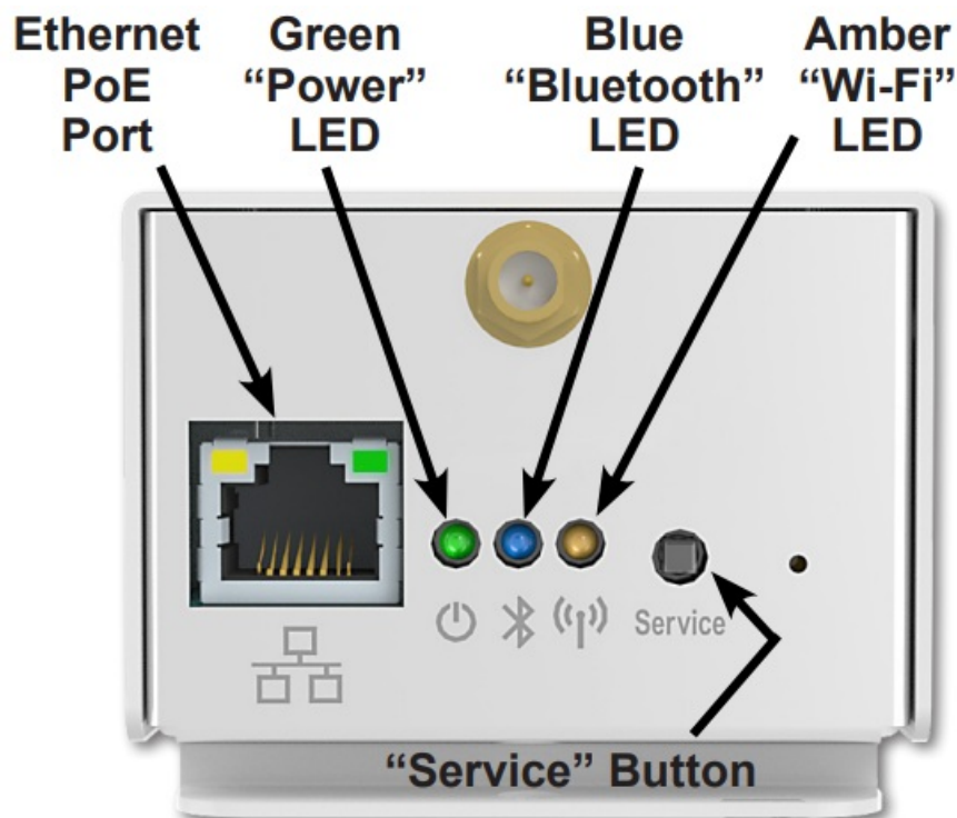
Fig. 1: Gateway PoE Port and LEDs
