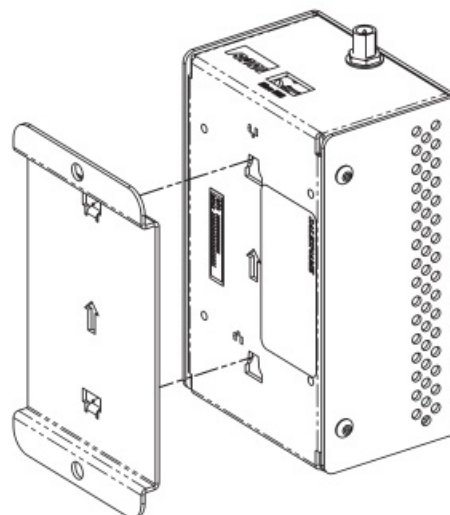
Fig. 10: Gateway mounting
