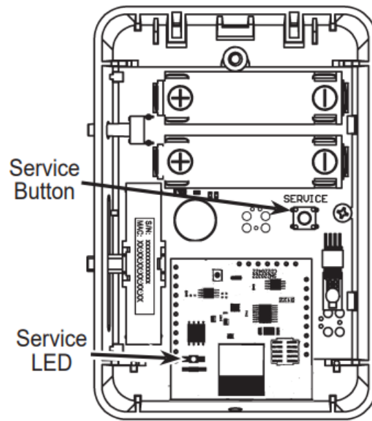
Fig. 9: BAPI-Stat "Quantum" Sensor Service Button and LED
