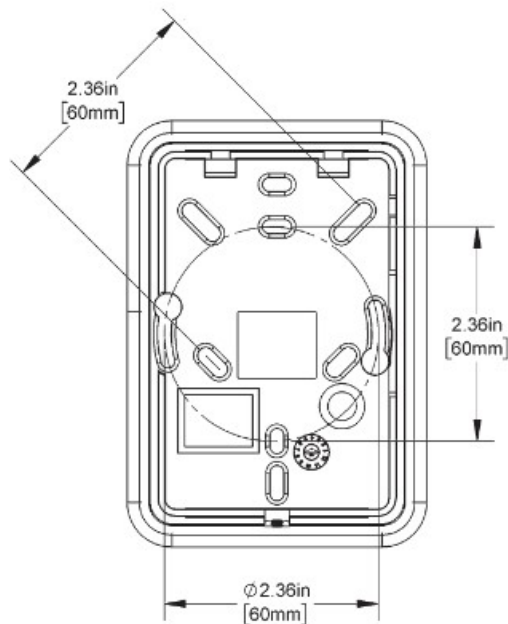
Fig. 4: 60mm mounting base dimensions
