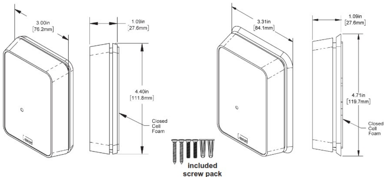
Fig. 1: BAPI-Stat "Quantum" CO Sensor
