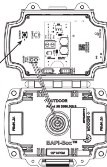
Fig. 5: Wire Power Unit
