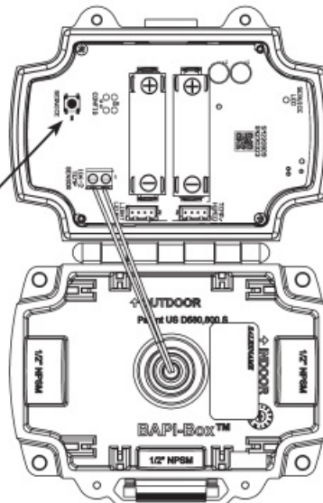
Fig. 4: Battery Power Unit
